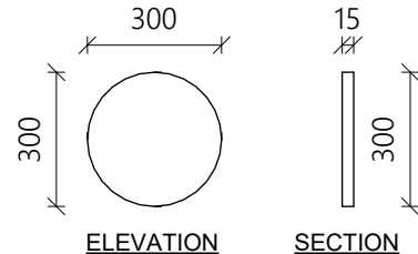
RECESS DETAIL
