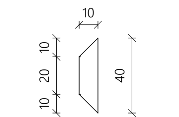
TYPICAL GROOVE DETAIL
