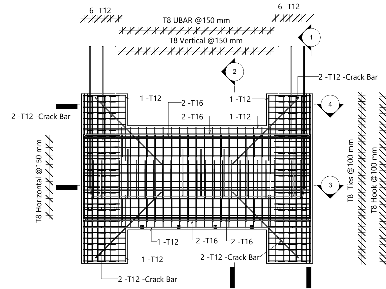
A ELEVATION(REINF) 1 : 40
