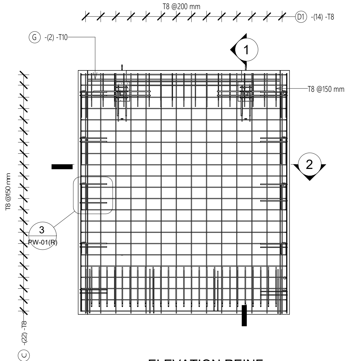
A ELEVATION REINF 1 : 30
