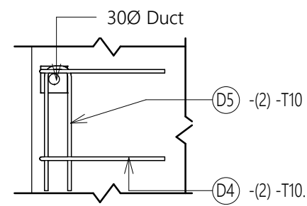
3 U-BAR DETAIL 1 : 15
