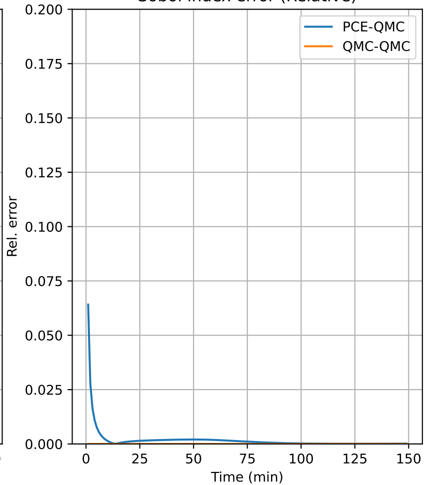
Sobol index error (Relative)
