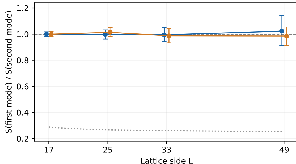
Lowest axis-mode transverse spectral trace
