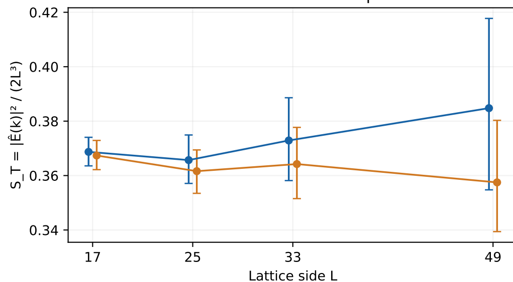
Lowest axis-mode transverse spectral trace
