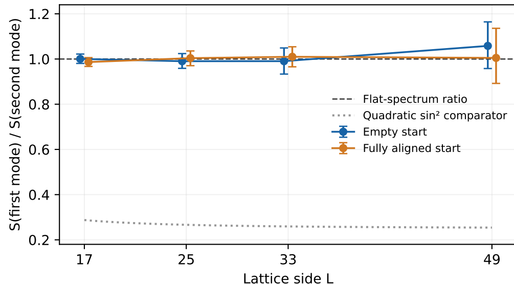
Occupation agrees across initializations
