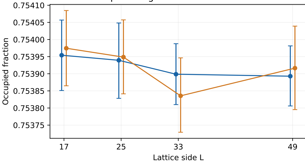
Occupation agrees across initializations
