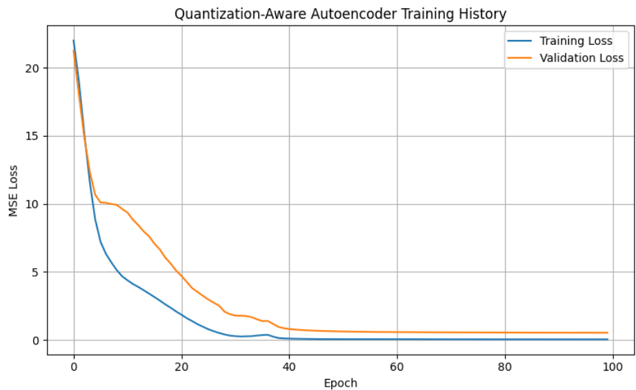
Quantization-aware autoencoder loss
