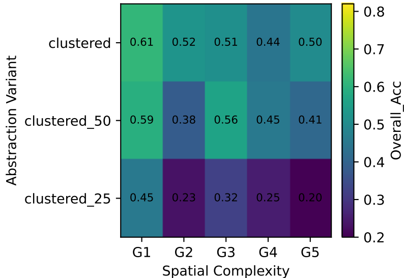
(b) Clustered family (Qwen3-32b)
