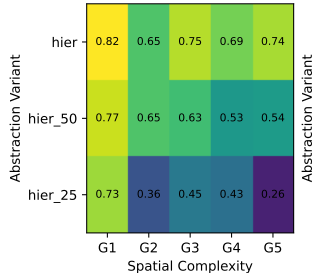
(a) Hierarchical family (Qwen3-32b)
