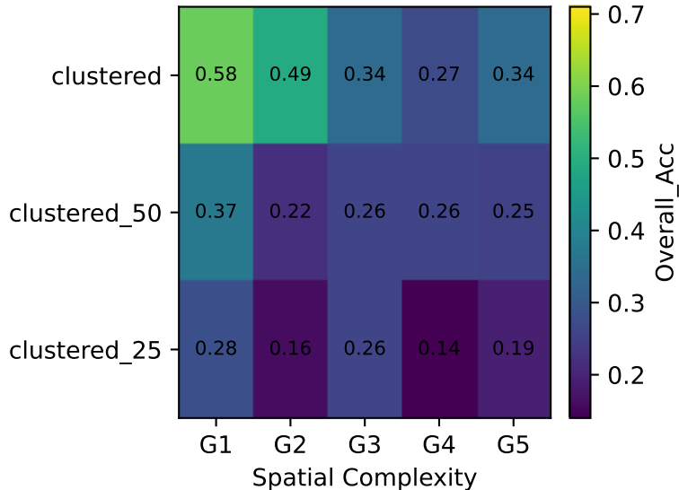
(b) Clustered family (Qwen3-4B)
