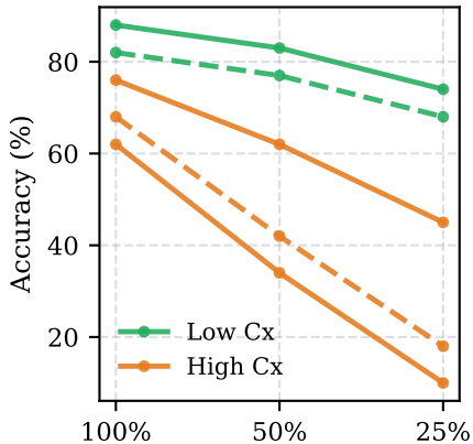
(2) Compression Resilience
