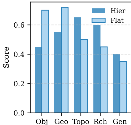
(3) Task Specialization
