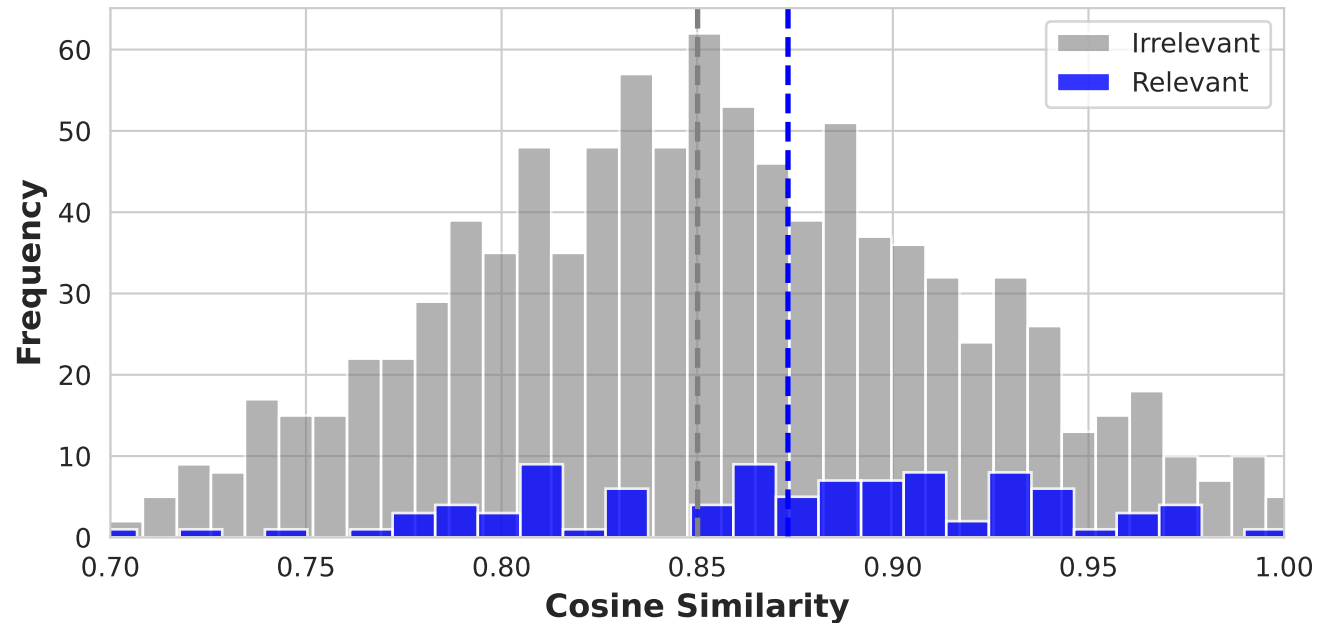
MiniLM: Normal Distribution (Discriminative Capacity Preserved)
