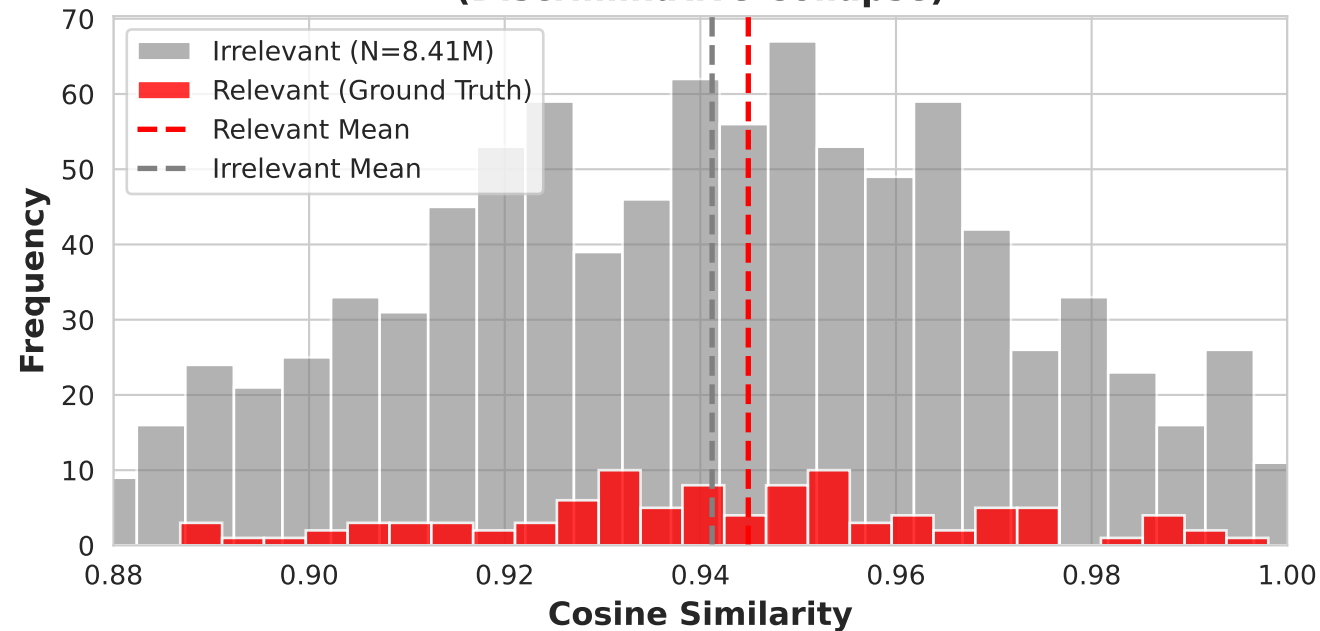
Math-BERT: Semantic Saturation (Discriminative Collapse)
