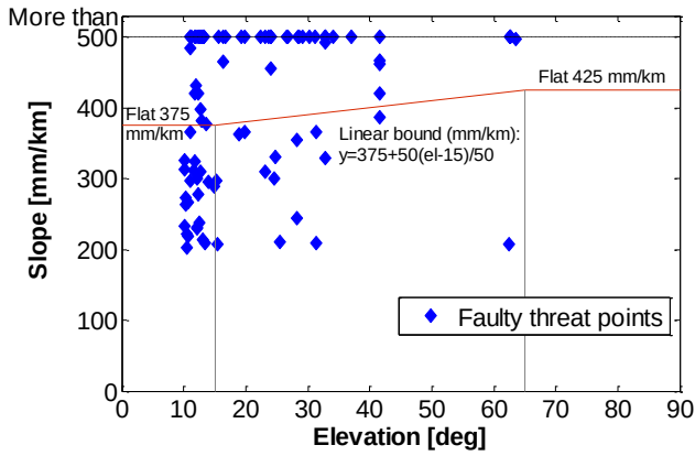
Figure 1. Faulty Candidates (92 points) Populated on Ionospheric Anomaly Threat Space Before Removing Stations with Poor GPS Data Quality on 26 May 2012.
