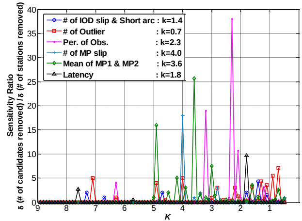
Figure 6 shows different sensitivity ratios with regards to the k value, which determines the reasonable threshold for all quality parameters. These sensitivity ratios are presented in different colors, and the label of Figure 6 shows the k values that maximize the sensitivity ratio of each parameter.
