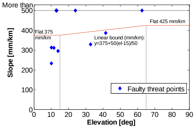
Figure 2. Faulty Candidates (11 points) Populated on Ionospheric Anomaly Threat Space After Removing Stations with Poor GPS Data Quality on 26 May 2012.
