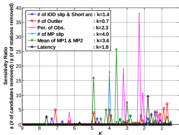
Figure 6. Sensitivity ratio for all quality parameters.
