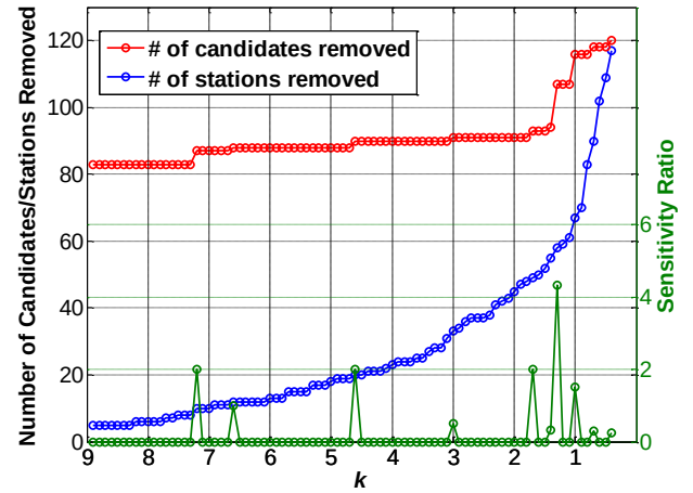
Figure 5. Comparison of number of candidates removed and stations removed and sensitivity ratio for IOD cycle slip.
