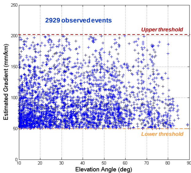
Figure 17. CONUS Ionospheric Gradients from LTIAM (50 to 200 mm/km)
