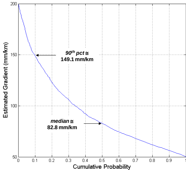
Figure 18. Cumulative Distribution of CONUS Ionospheric Gradients from LTIAM (50 to 200 mm/km)
