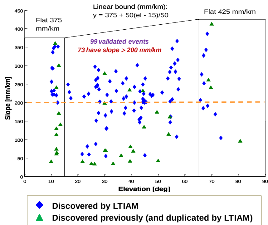
Figure 16. CONUS Ionospheric Threat Model with Observed Spatial Gradients (LTIAM Threshold = 200 mm/km)
