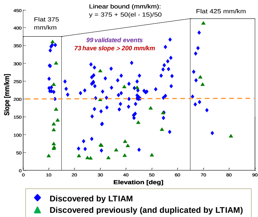
Figure 16. CONUS Ionospheric Threat Model with Observed Spatial Gradients (LTIAM Threshold = 200 mm/km)
