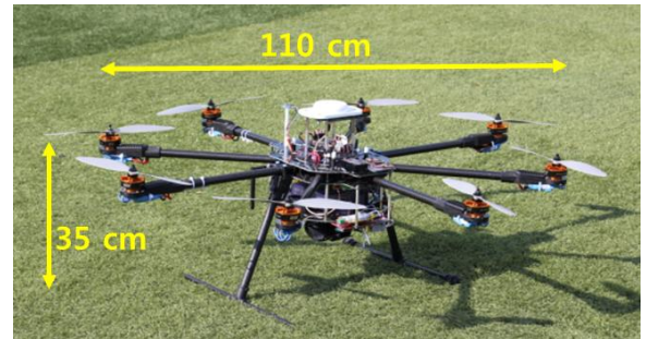
Figure 9. Multi-copter UAV Platform for Flight Test
