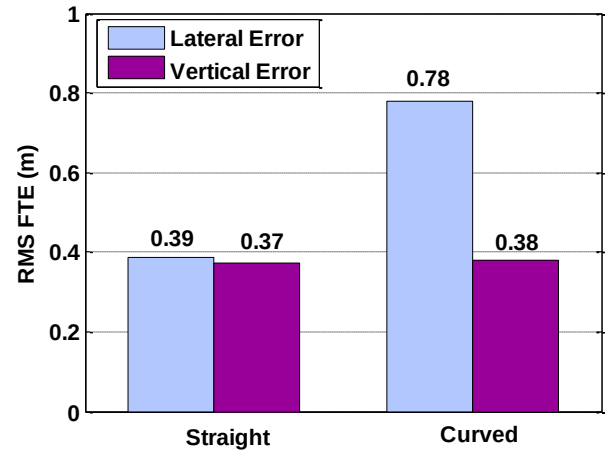
Figure 11. Flight Technical Error: Straight vs. Curved Segments
