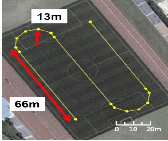
Figure 5. Flight Path of UAV Flight Experiments
