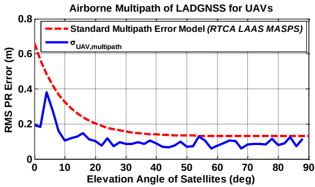
Figure 10. Observed UAV Multipath Compared with Standard Model.
