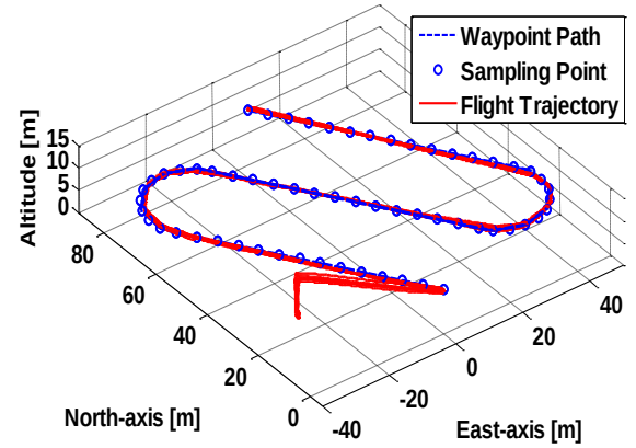
Figure 6. Waypoint Path (Defined Guidance path), Flight Trajectory (Estimated Position) and Sampling Points with Constant Interval
