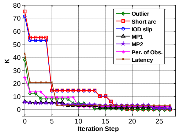
Figure 10. K Values of All Seven Quality Parameters
