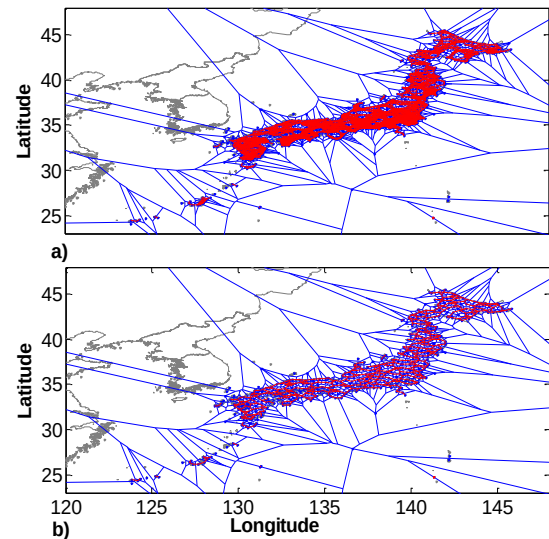
Figure 16. Map of Voronoi Diagram of GEONET Stations with Baseline Constraint of 40 km: a) Before Subset Selection Processing b) After Subset Selection Processing (Baseline in Red; Voronoi Region in Blue Polygon)
