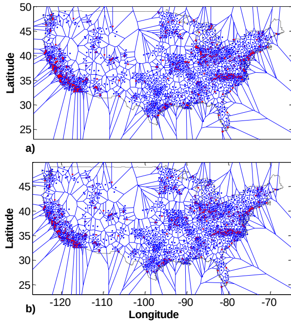
Figure 13. Voronoi Diagram of CORS Stations with Baseline Constraint of 40 km: a) Before Subset Selection Processing b) After Subset Selection Processing (Baselines in Red; Voronoi Regions in Blue Polygon)
