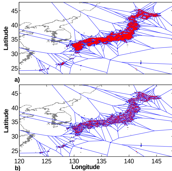
Figure 16. Voronoi Diagram of GEONET Stations with Baseline Constraint of 40 km: a) Before Subset Selection Processing b) After Subset Selection
