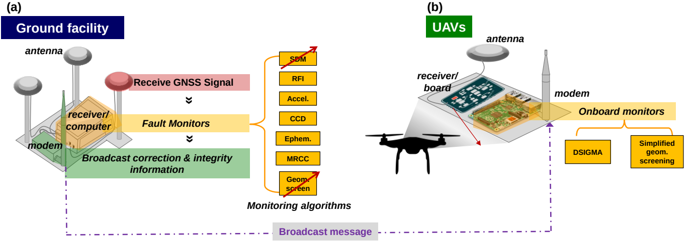
Figure 3. Configuration and components of the LAD-GNSS architecture
