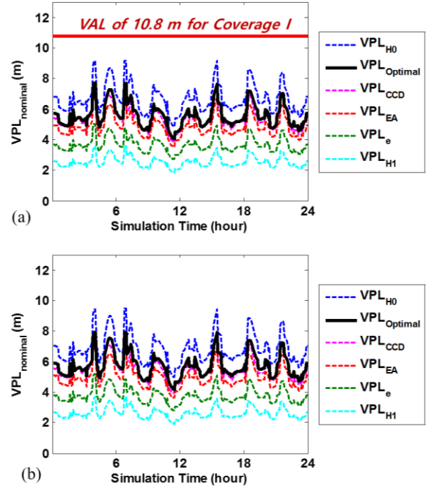
Figure 7. VPLs of LAD-GNSS for UAV operating in (a) Coverage I and (b) Coverage II
