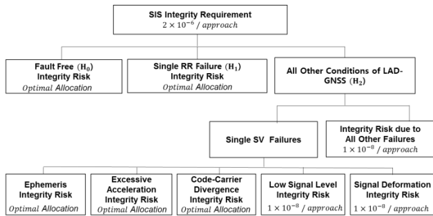
Figure 5. Integrity risk allocation of LAD-GNSS for UAVs
