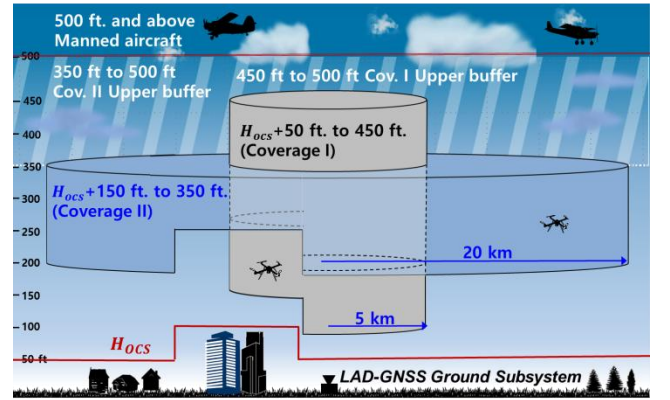
Figure 2. LAD-GNSS architecture for UAV (when H_{OCS} are assumed)
