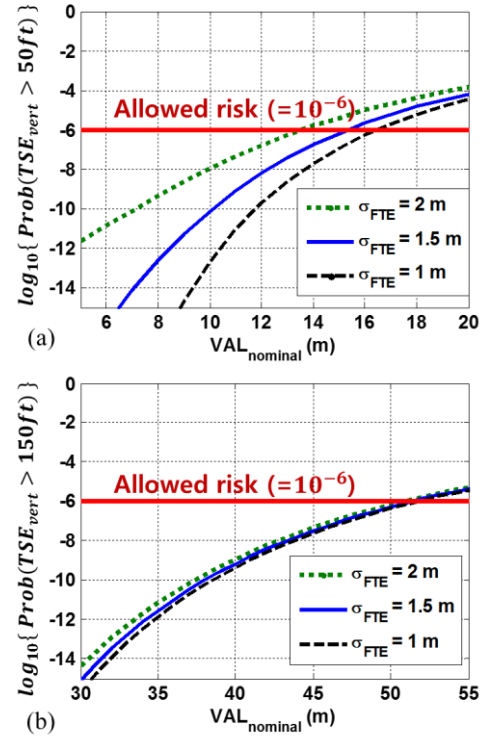
Figure 4. Probability that TSE_{vert} is greater than (a) 50 ft for Coverage I and (b) 150 ft for Coverage II
