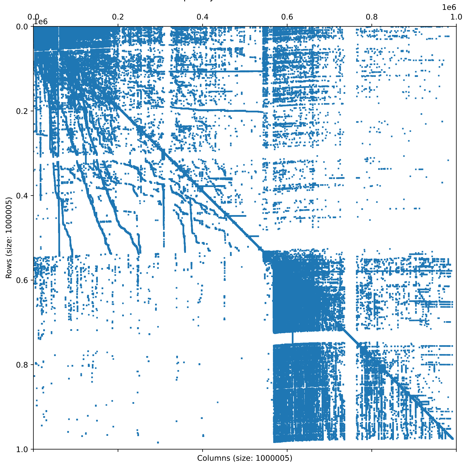
Sparsity Pattern of the Matrix
