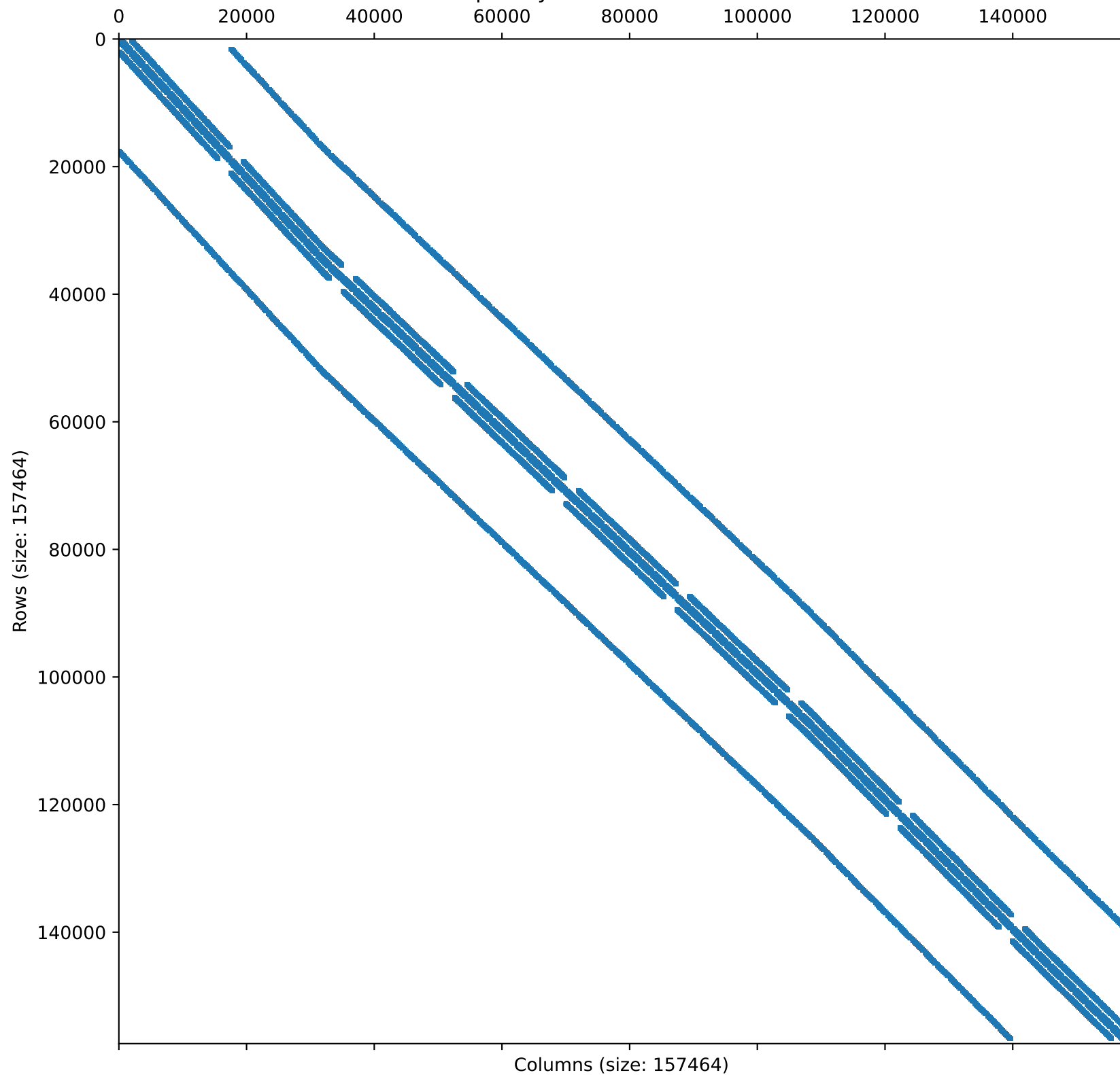
Sparsity Pattern of the Matrix
