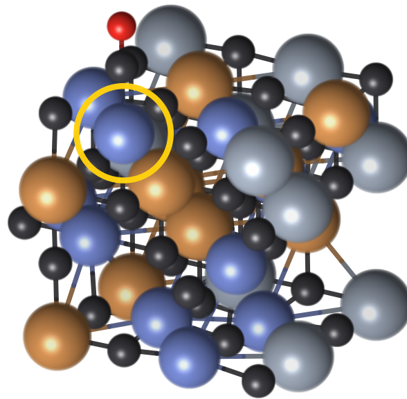
(b) (Cr, Ti, V)C
