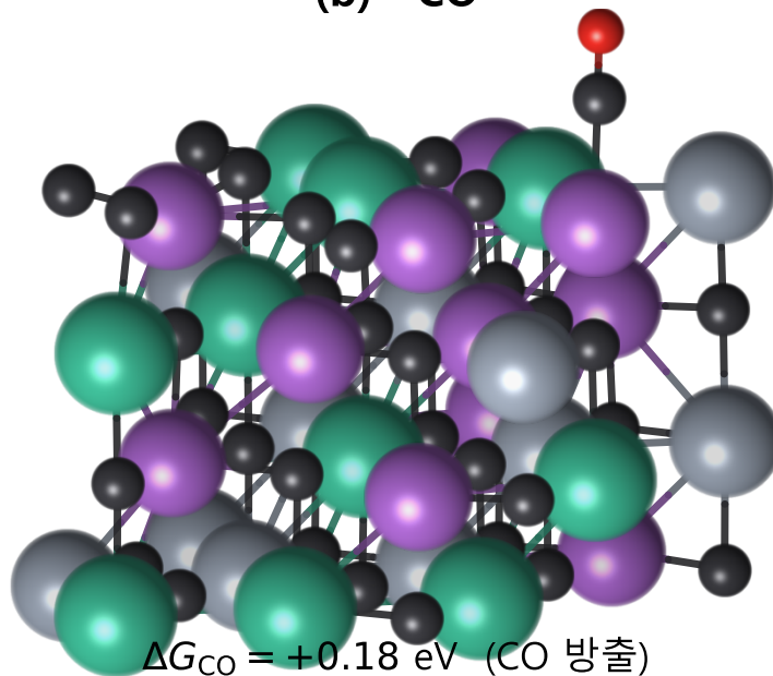
(b) *CO
