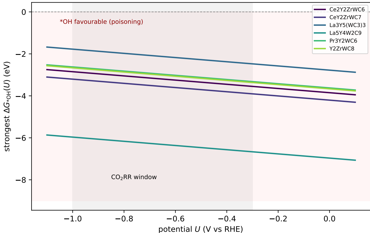
Surface Pourbaix: *OH binding vs potential (UMA, strongest site)
