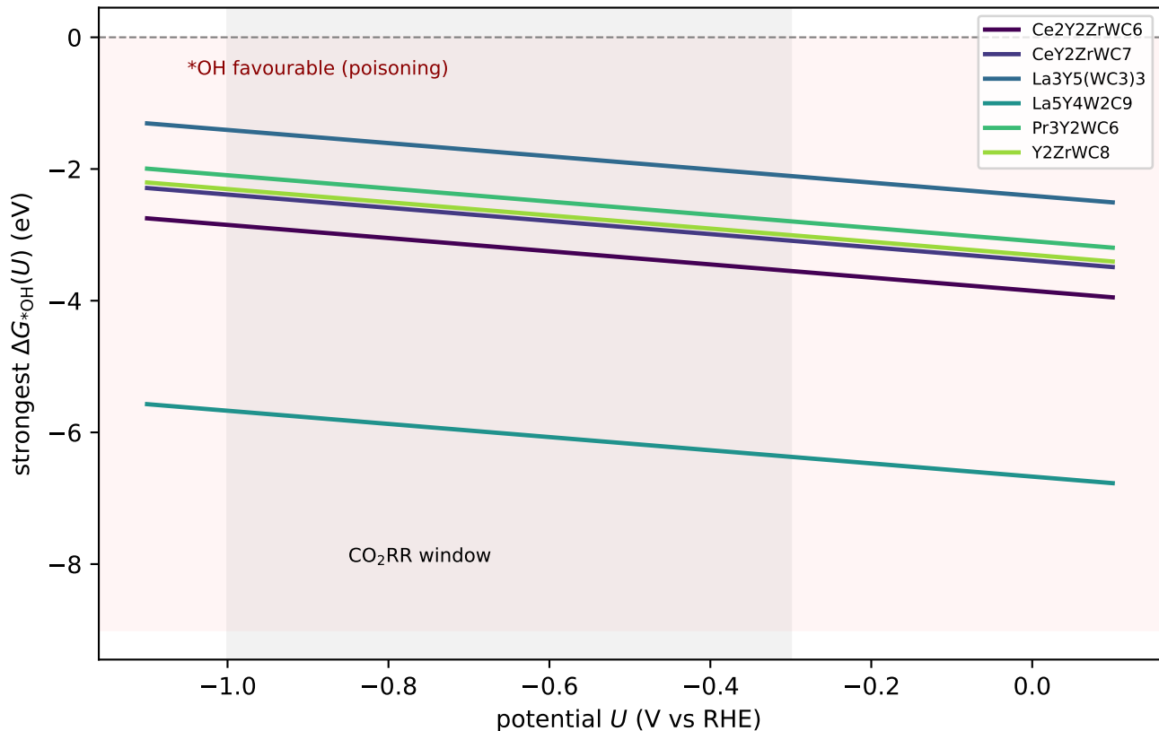
Surface Pourbaix: *OH binding vs potential (DFT, strongest site)
