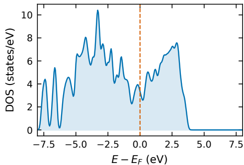
CeY2ZrWC7 DOS( E_F )=3.3
