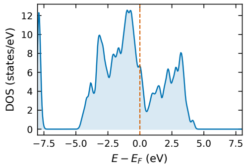
Ce2Y2ZrWC6 DOS( E_F )=6.7
