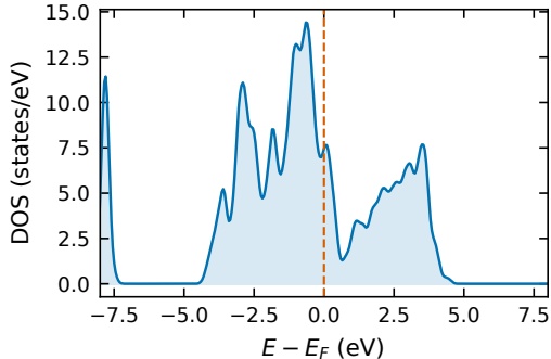
Pr3Y2WC6 DOS( E_F )=7.4
