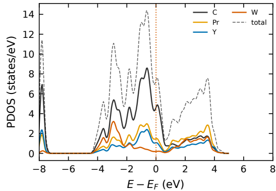
Pr3Y2WC6
