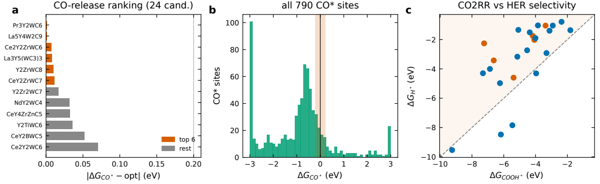
Figure 4.4: UMA surface screen: (a) candidates ranked by proximity of the best site to the CO optimum; (b) pooled \Delta G_{CO^*} distribution with the CO-release window; (c) CO-vs- H_2 selectivity ( \Delta G_{COOH^*} versus \Delta G_{H^*} ).
