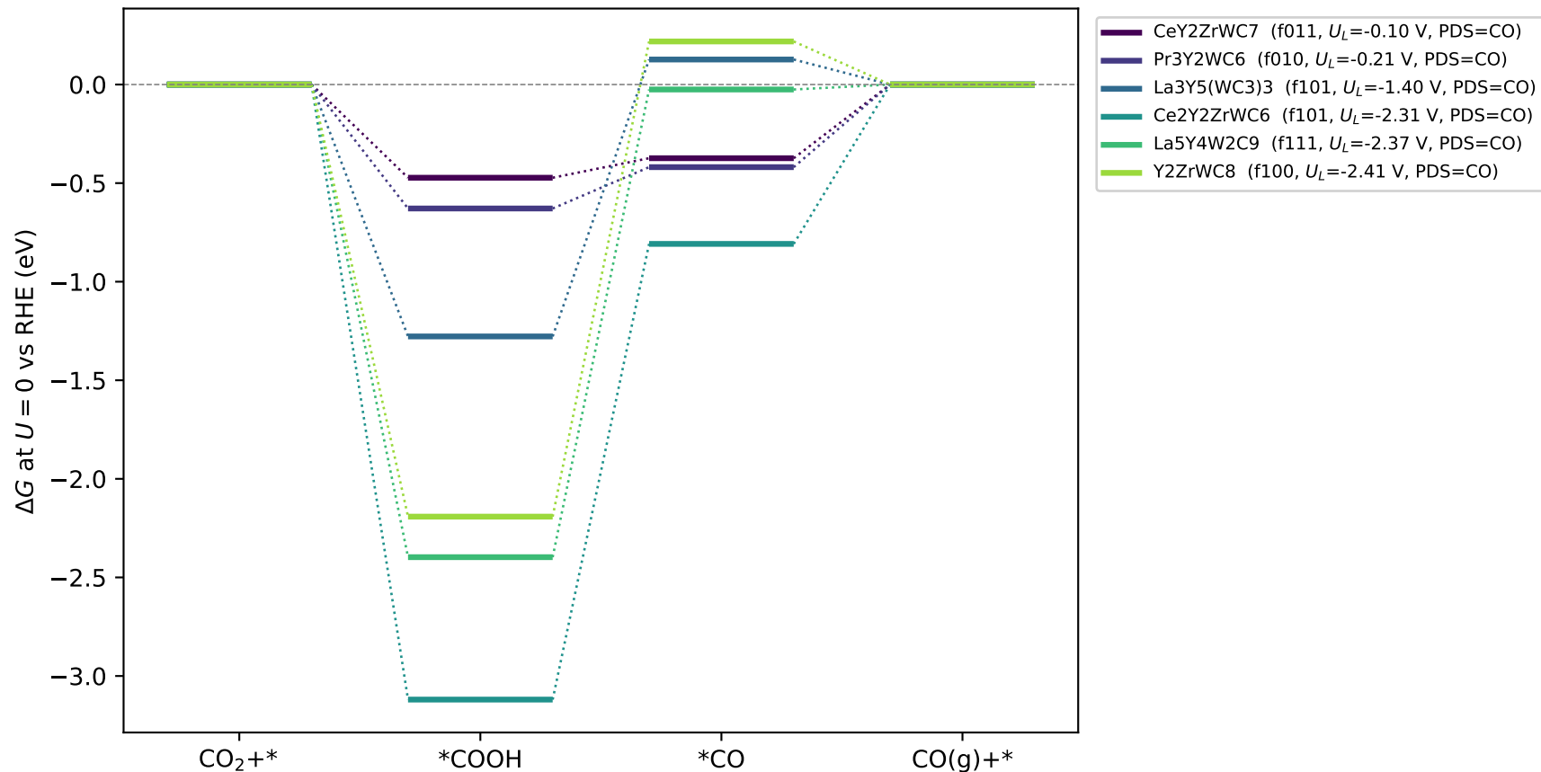
CO 2 RR-to-CO free-energy diagram (DFT, best facet per candidate)
