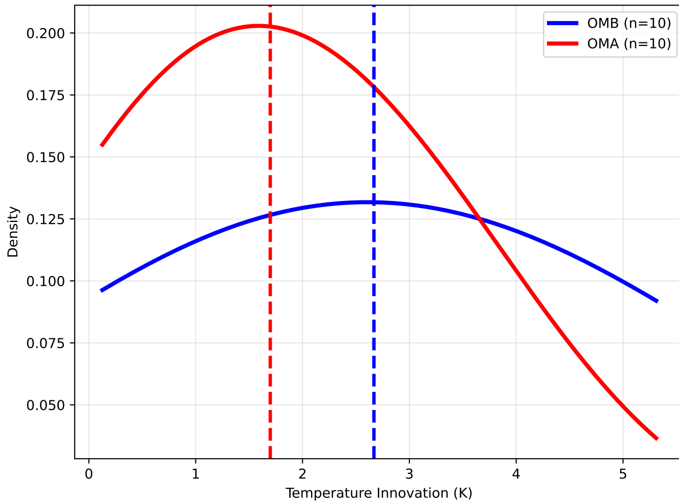
OMB (Blue) vs OMA (Red) RMSE: 3.22 \rightarrow 2.06 K
