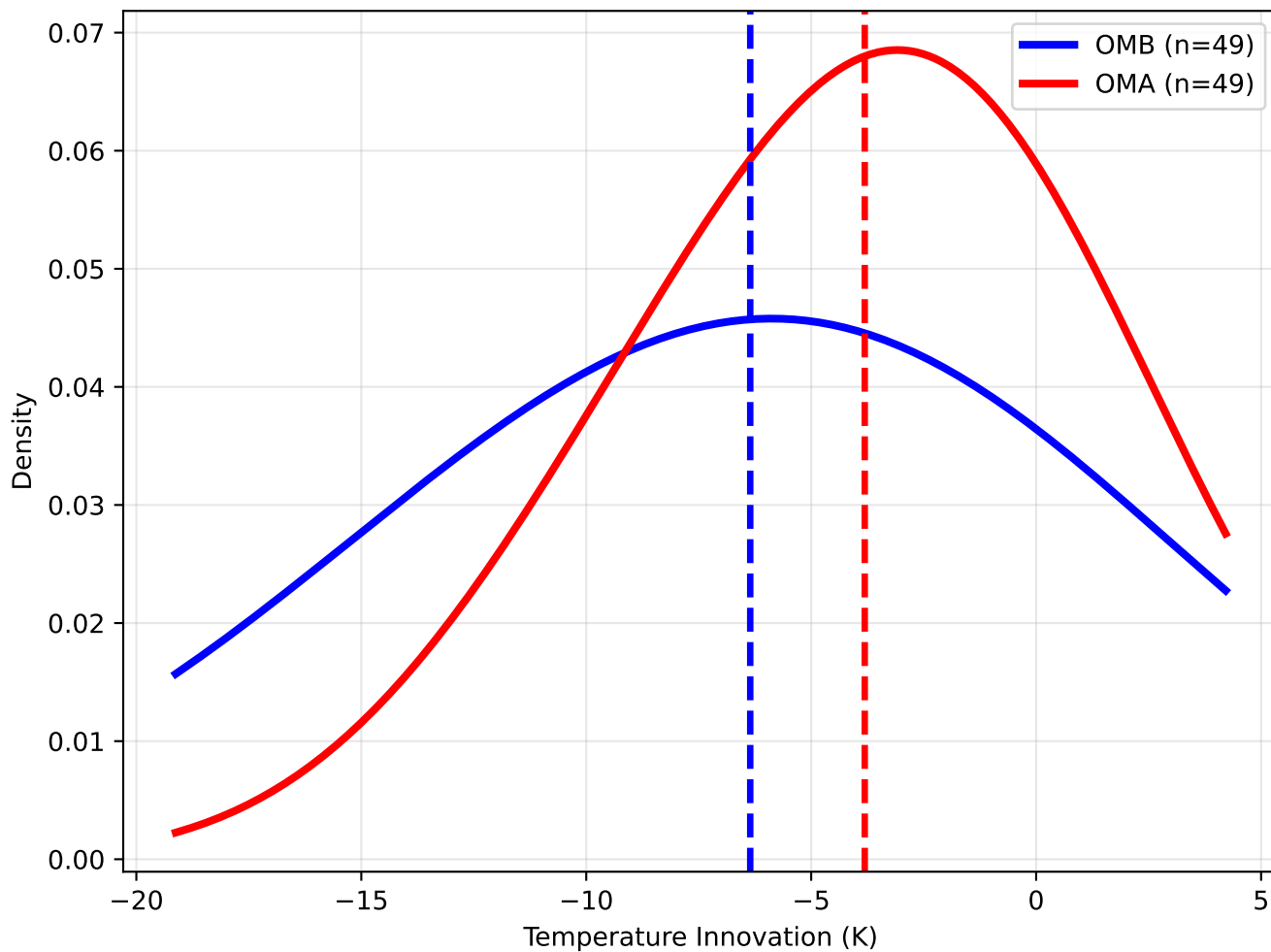
OMB (Blue) vs OMA (Red) RMSE: 8.37 \rightarrow 5.28 K
