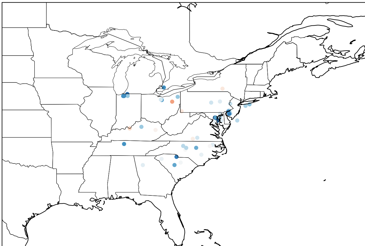
OMB (Obs - Background)
