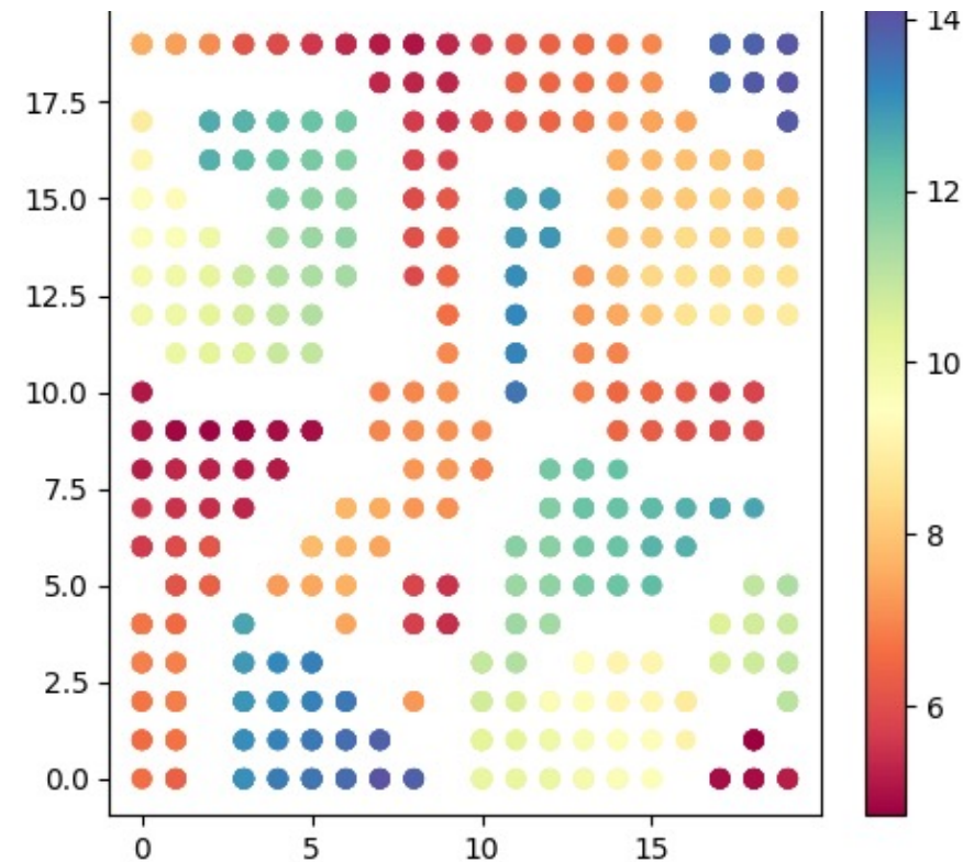
low-D space
