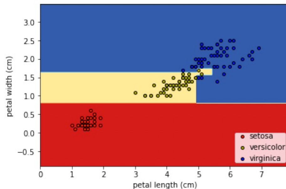
Decision surface of decision tree
