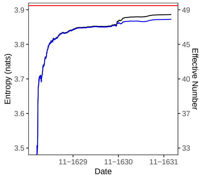
a Entropy of invCDF
