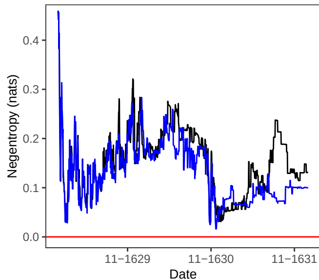
b Negentropy of PDF
