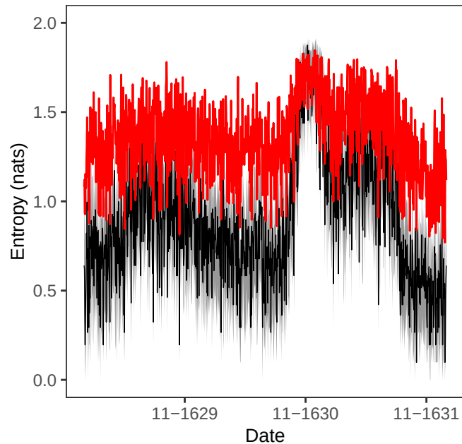
a Entropy
