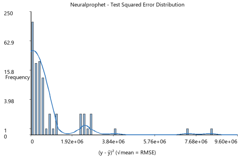
FIGURA 4.3. RMSE Neural prophet.
