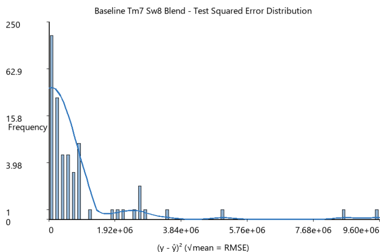
FIGURA 4.5. RMSE baseline .
