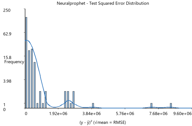
FIGURA 4.3. RMSE NeuralProphet.
