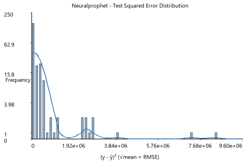
FIGURA 4.3. RMSE Neuralprophet.
