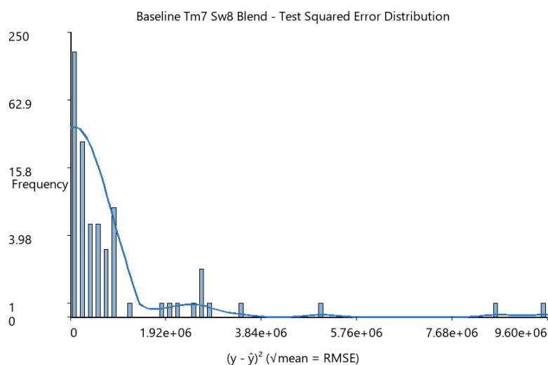
FIGURA 4.3. RMSE Baseline .
