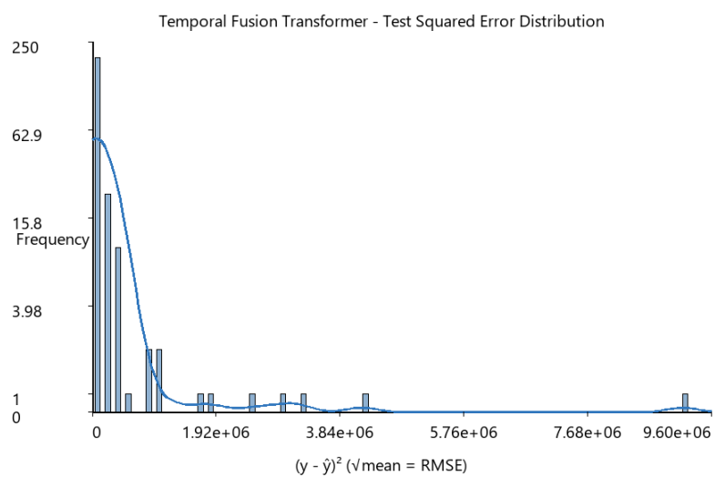
FIGURA 4.5. RMSE TFT.
