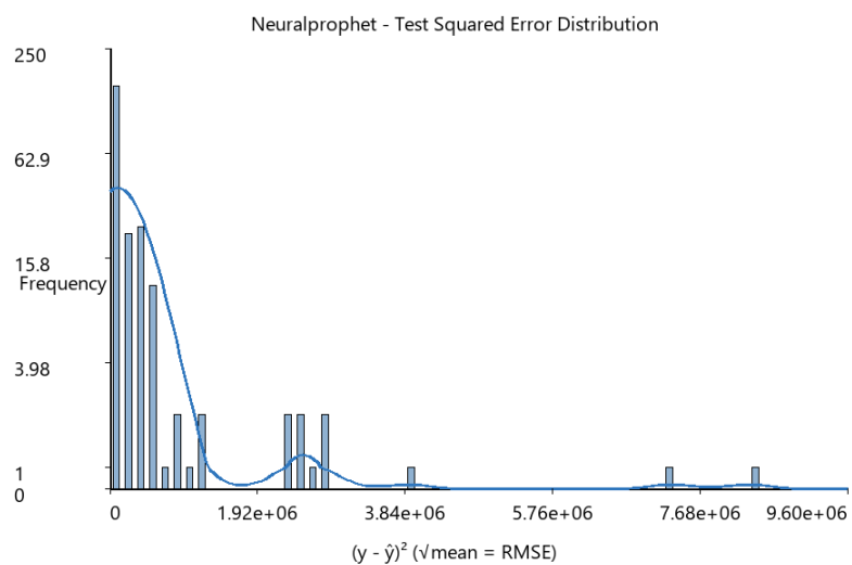
FIGURA 4.4. RMSE Neural prophet.
