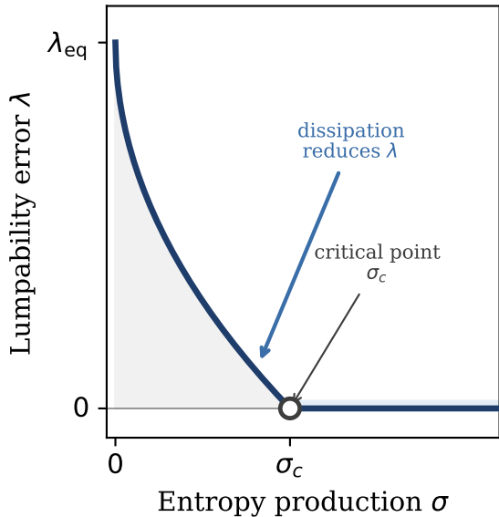
(a) Dissipation-lumpability
