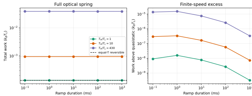
Figure 2: Predicted work for the 85 to 58 Hz change. Left: total mechanical work. Right: work above the steady-state path integral, which is a free-energy difference only for equal-temperature baths. These curves are model predictions, not measured apparatus power.
