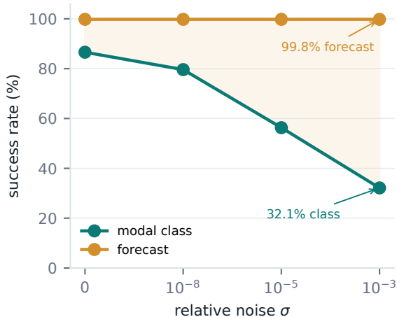
Prediction survives a false explanation
