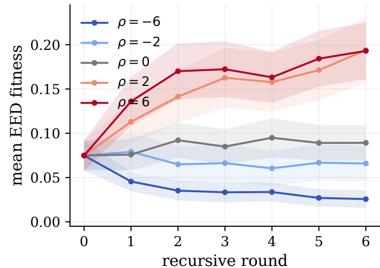
A. Continuous solution fitness
