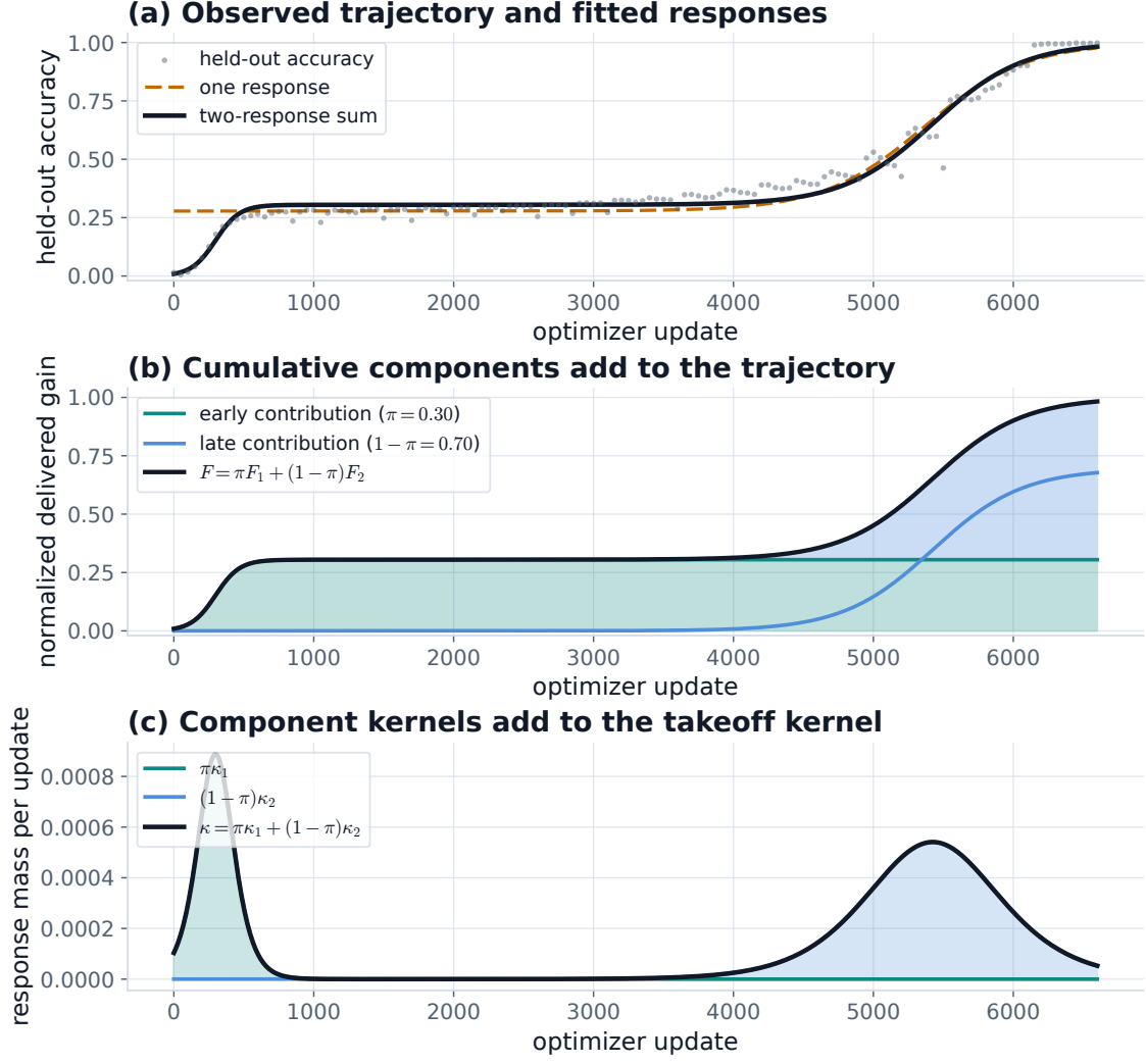
Figure 2: Anatomy of the fitted response. (a) For representative seed 20260803, one response absorbs the early plateau into a baseline; two responses follow the data. (b) The early and late cumulative contributions add to the normalized trajectory. (c) Their weighted kernels add pointwise to the final takeoff kernel. This is the parallel mixture (6), not a demonstrated sequential convolution (7).
