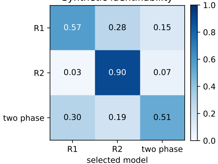
Synthetic identifiability
