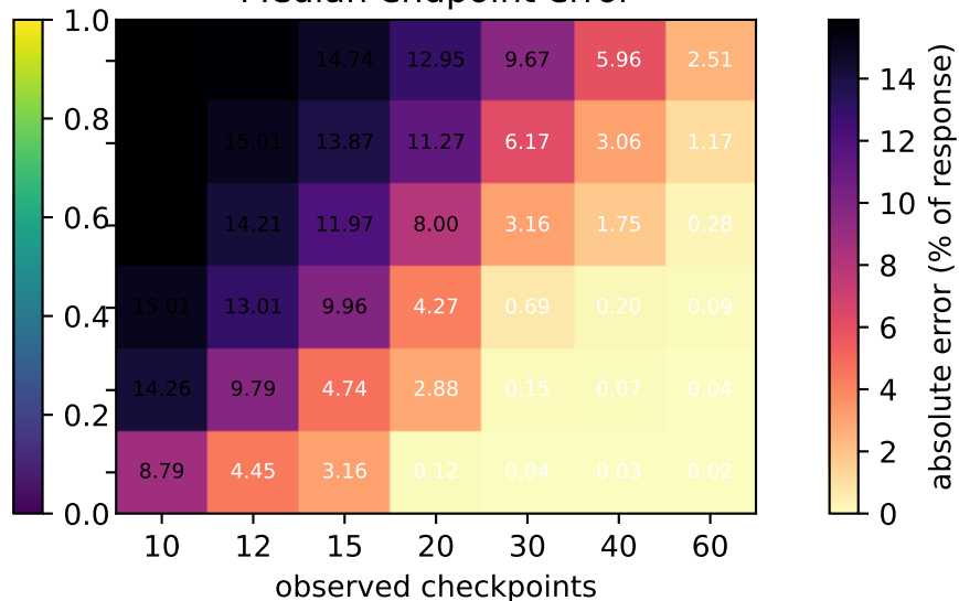
Median endpoint error
