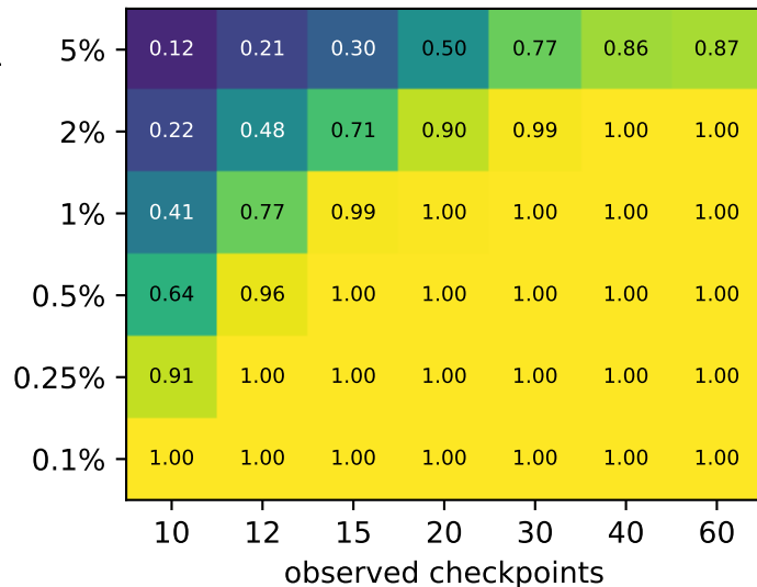
Held-out rank-two detection
