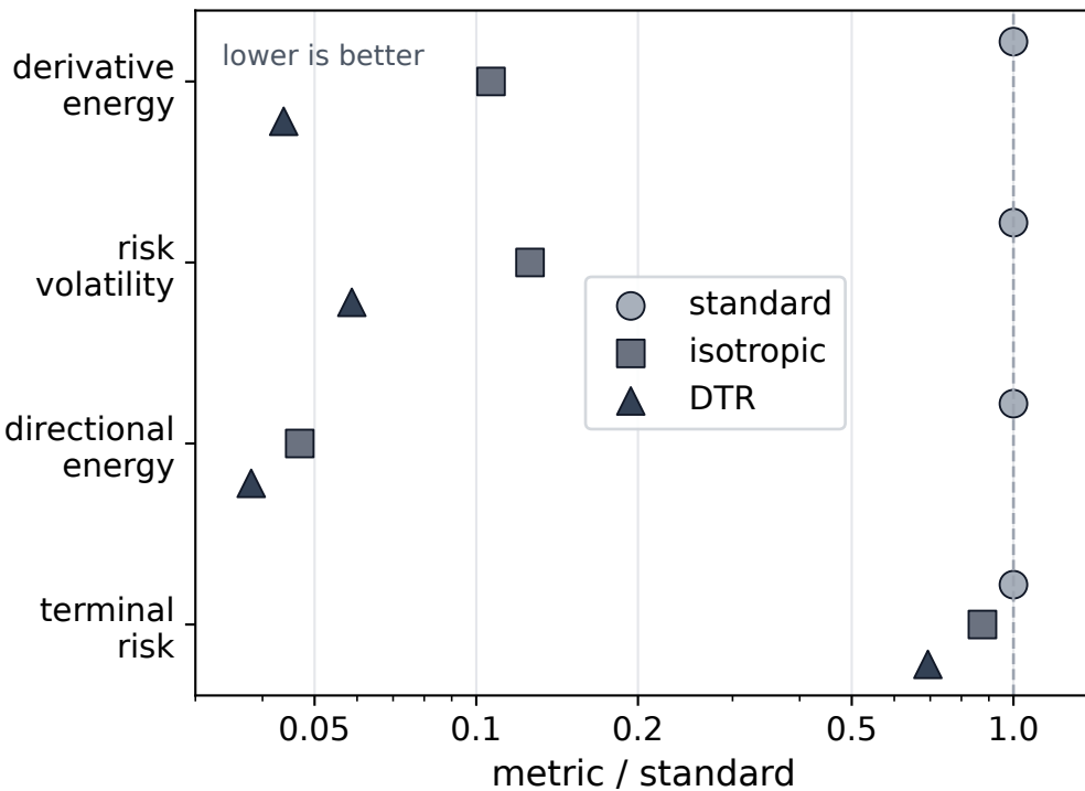
Matched \lambda = 0.03 comparison
