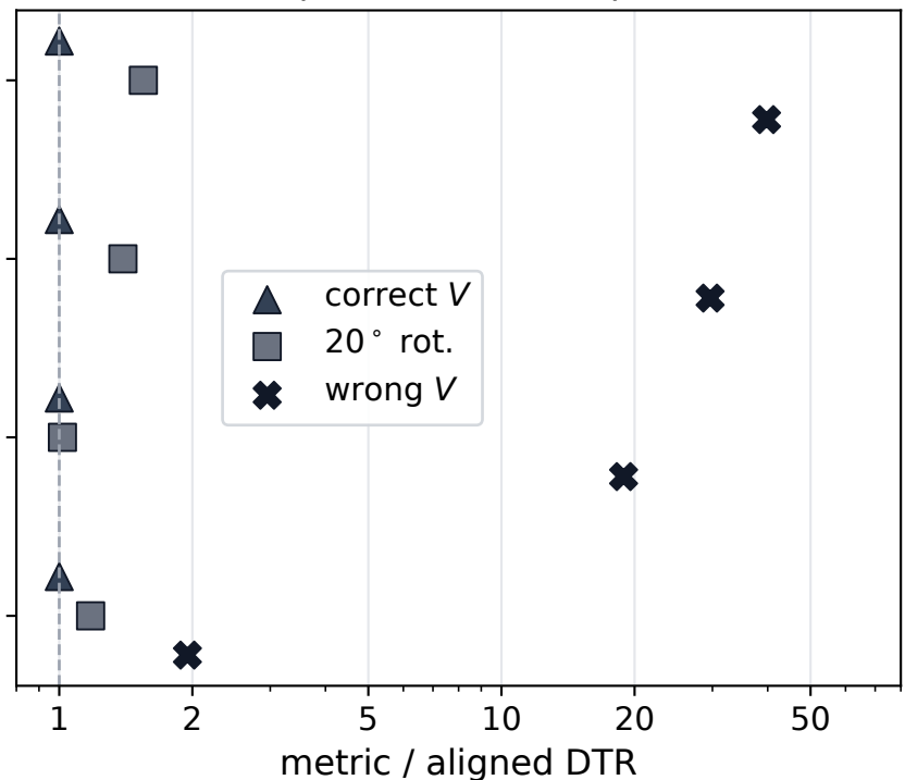
Misspecified drift subspace
