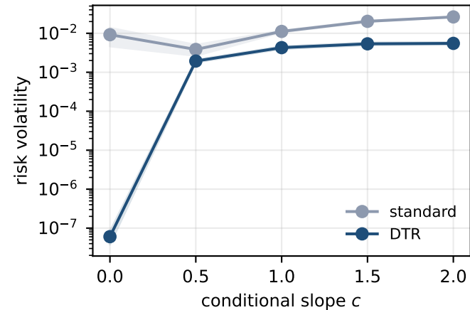
Conditional variation limits tangent control
