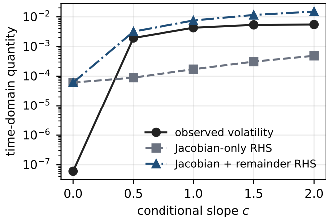
The remainder restores valid control
