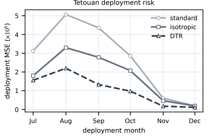
Fig. 5. Tetouan frozen deployment over six monthly blocks. DTR stays below both standard and isotropic training throughout the deployment horizon, with the largest gap in the late-summer high-risk regime.
