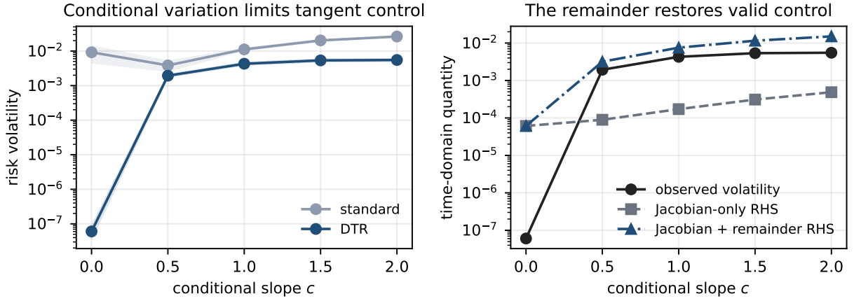
Fig. 4. Conditional-risk remainder stress test. Left: DTR nearly removes volatility when the label conditional is spatially constant, but volatility returns as its slope c grows. Right: for DTR, the Jacobian-only right-hand side fails for every run with c > 0 , while the coupled Jacobian-plus-remainder bound remains valid. Curves show means over 100 seeds; shading shows 95% confidence intervals for the mean.
