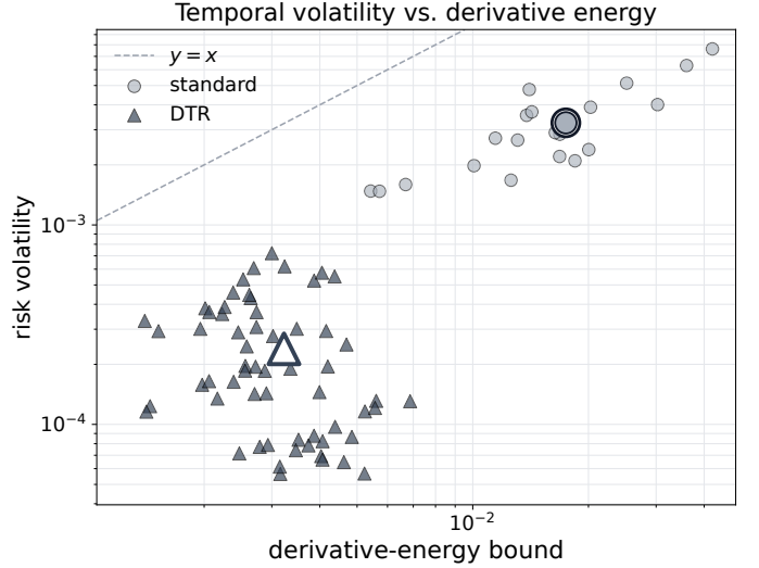
Fig. 2. Synthetic time-domain sanity check on log-log axes. Each point is one trained model evaluated over the drifting deployment path. The horizontal axis is the derivative-energy quantity from Lemma 1 and (3), and the vertical axis is empirical volatility \text{Var}_U(r(U)) . Large outlined markers denote method means. DTR shifts models toward lower energy and lower volatility.
