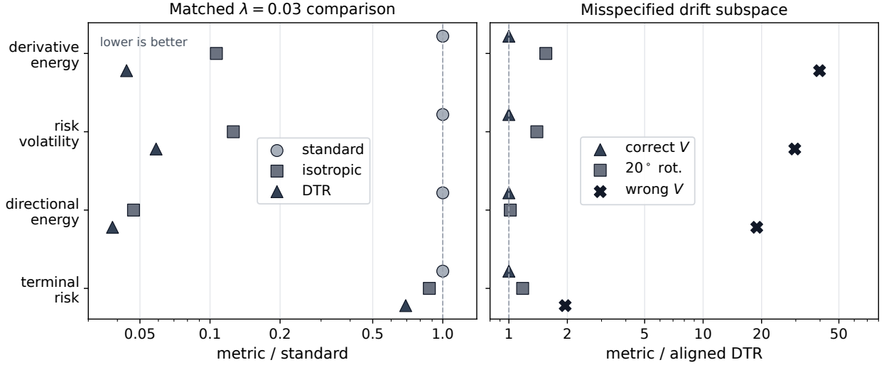
Fig. 3. Synthetic directional comparisons. Left shows matched \lambda = 0.03 ratios for derivative energy, risk volatility, directional energy, and terminal risk, normalized by the standard model. DTR is lower than isotropic Jacobian regularization on all four metrics. Right shows the same metrics normalized by aligned DTR for the correct subspace, a mild 20^\circ rotation, and a wrong subspace. Mild misspecification is tolerable, but wrong subspaces are not.
