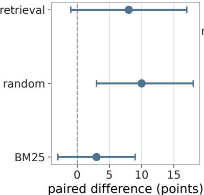
(b) Semantic gain at k = 3
