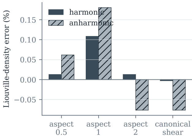
Phase volume forgets the grid
