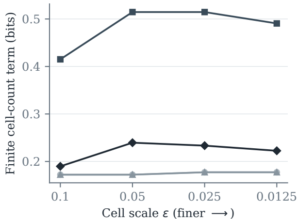
Cell incidence retains the grid
